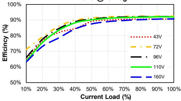
CQB100W-110S12 Eff Vs Io @25 Deg. C
