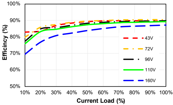
CQB100W-110S24 Eff Vs Io @25 Deg. C
