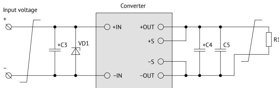
Figure 2. MDRW50 typical connection diagram.
