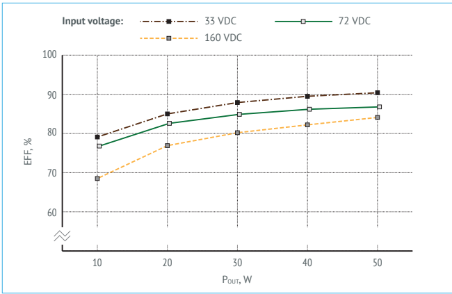
Figure 18. Efficiency.
