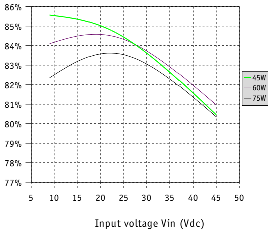
Typical efficiency MGDS-75-H-E at 25°C
