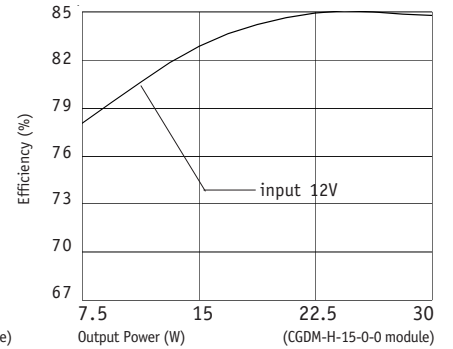
Figure 6 : Typical efficiency versus load at various input
