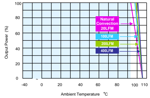
AER10-48D12 Derating Curve with Heatsink
