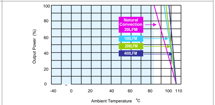
AER10-110S05 Derating Curve with Heatsink
