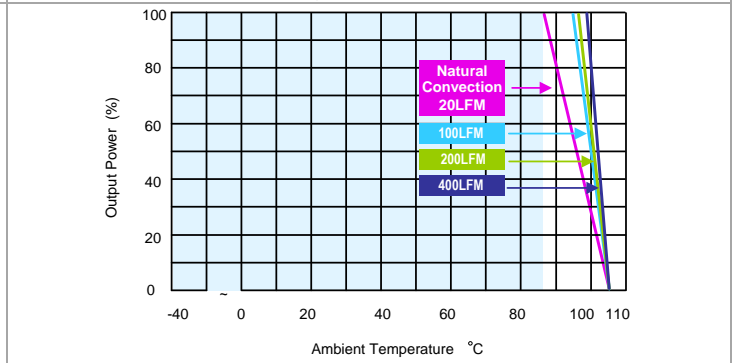
AER10-24S05 Derating Curve with Heatsink
